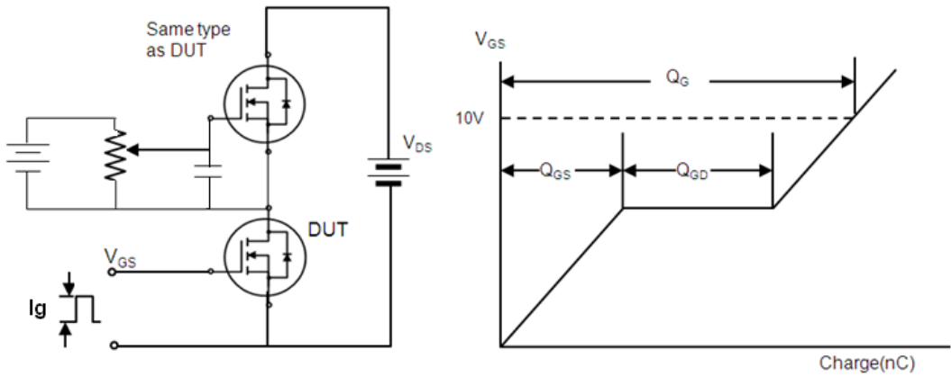
Fig. 16. Switching time test circuit & waveform
