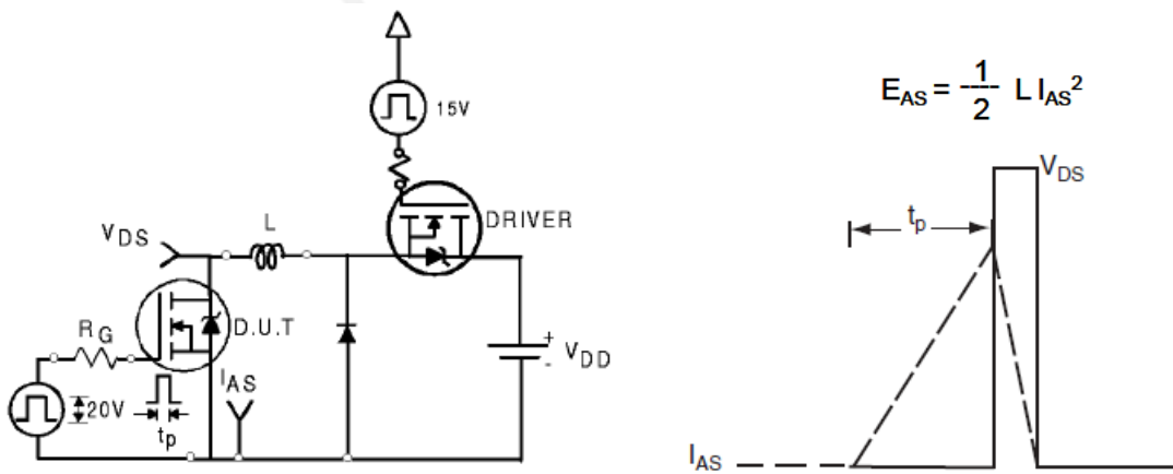
Fig. 17. Unclamped Inductive switching test circuit & waveform
