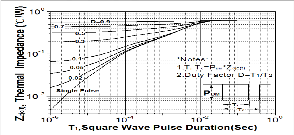
Fig. 10. Transient thermal response curve(TO-252&TO-251)
