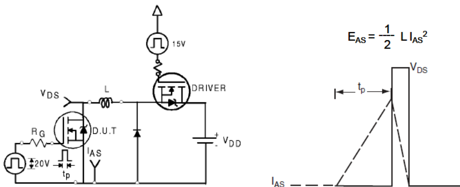
Fig. 18. Unclamped Inductive switching test circuit & waveform
