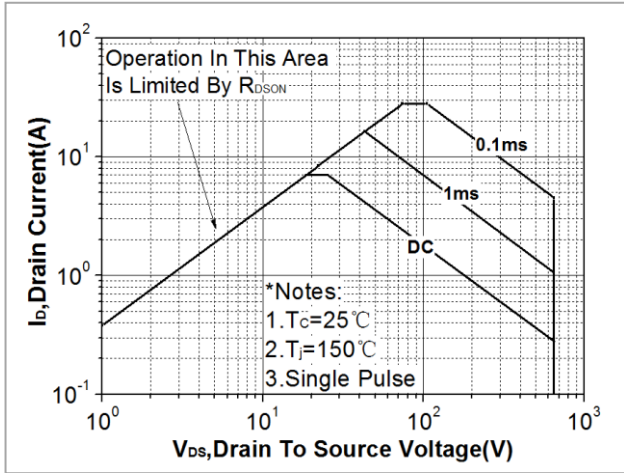
Fig. 12. Maximum safe operating area(TO-262N)
