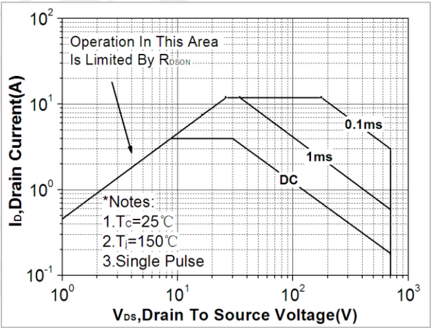
Fig. 10. Maximum safe operating area (TO-251N)
