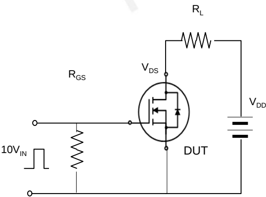
Fig. 14. Switching time test circuit & waveform
