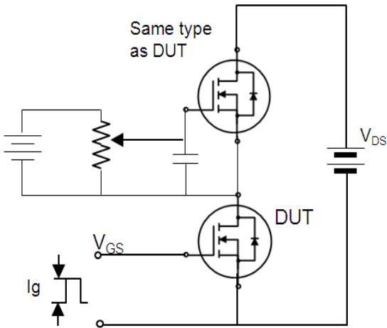
Fig. 13. Gate charge test circuit & waveform
