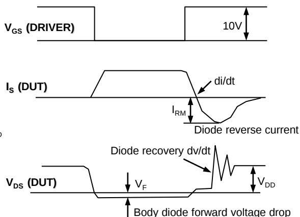
Fig. 17. Peak diode recovery dv/dt test circuit & waveform
