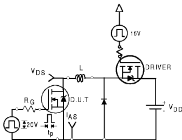
Fig. 16. Unclamped Inductive switching test circuit & waveform
