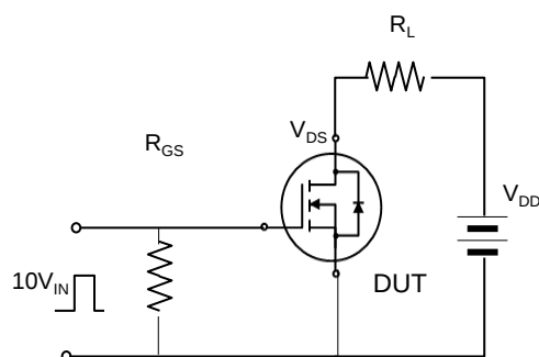
Fig. 15. Switching time test circuit & waveform
