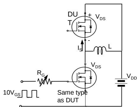
Fig. 17. Peak diode recovery dv/dt test circuit & waveform
