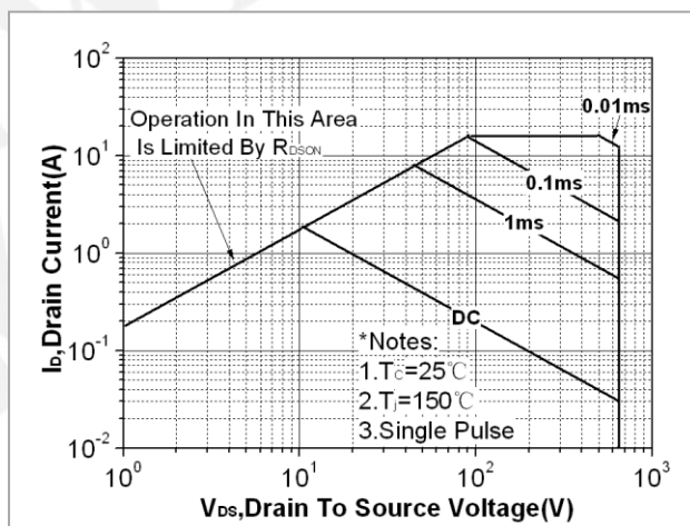
Fig. 10. Maximum safe operating area (TO-220F/TO-220SF)
