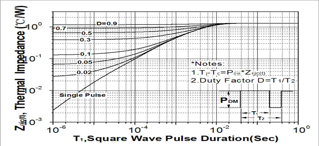
Fig. 12. Transient thermal response curve(TO-252&TO-251S)
