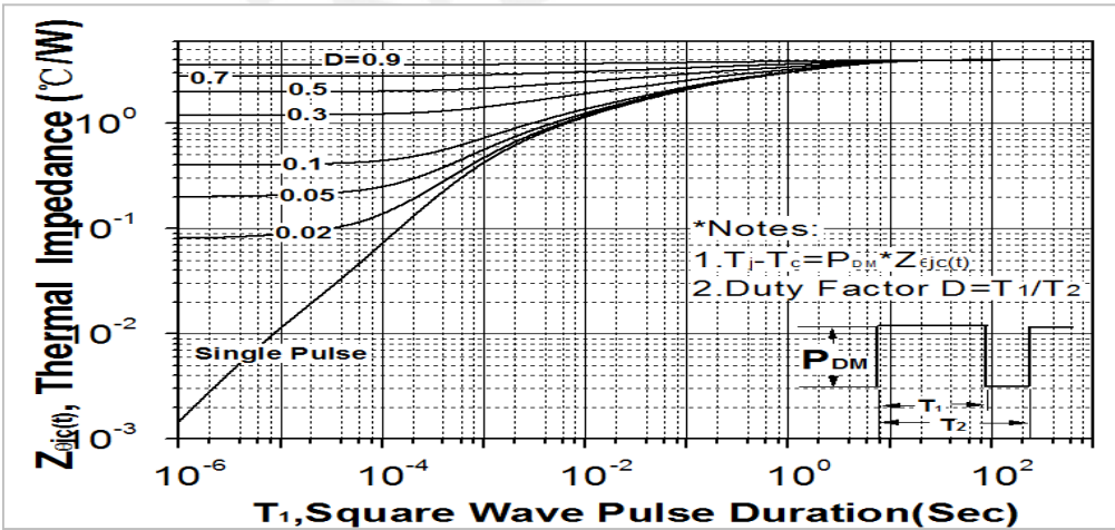
Fig. 11. Transient thermal response curve(TO-220F)
