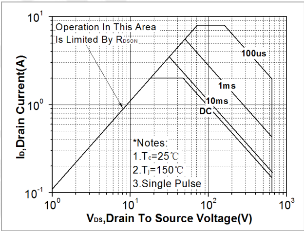
Fig. 10. Maximum safe operating area (TO-252&TO-251S)
