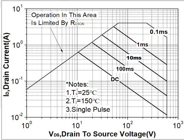
Fig. 10. Maximum safe operating area(SOT223)
