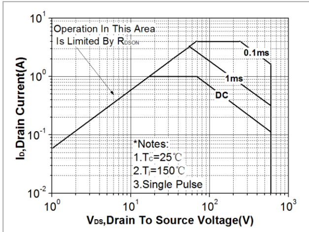
Fig. 7. Maximum safe operating area (TO-251)
