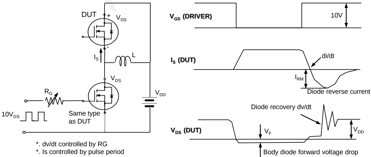
Fig. 17. Peak diode recovery dv/dt test circuit & waveform
