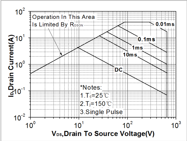
Fig. 9. Maximum safe operating area (TO-220F&TO-220FT)
