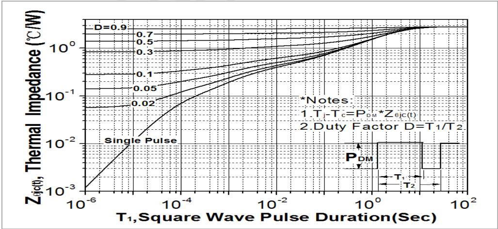
Fig. 10. Transient thermal response curve(TO-220F&TO-220FT)
