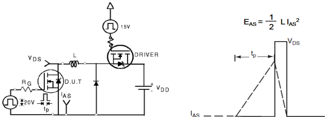
Fig. 13. Unclamped Inductive switching test circuit & waveform
