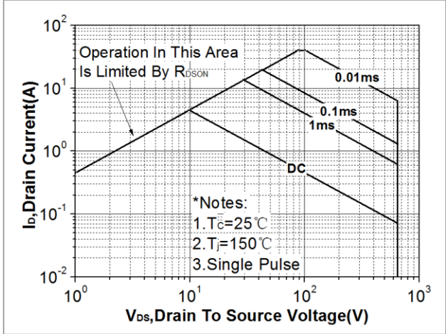
Fig. 7. Maximum safe operating area (TO-220F/TO-220SF/TO-220FT)
