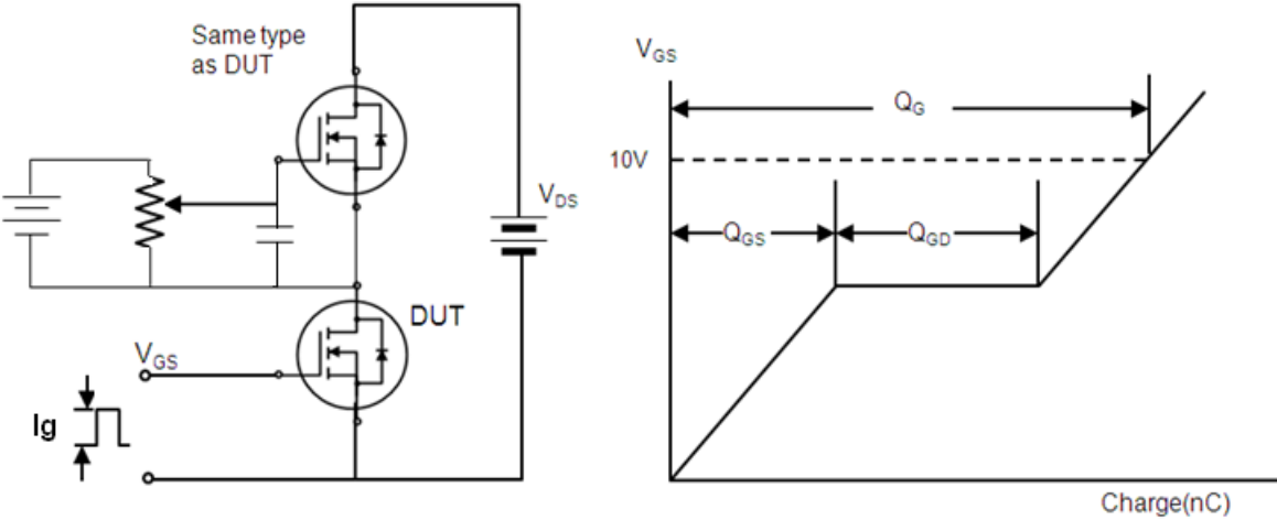
Fig. 15. Gate charge test circuit & waveform
