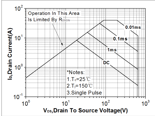
Fig. 9. Maximum safe operating area (TO-262/TO-262N)
