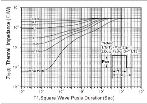
Fig. 9. Transient thermal response curve
