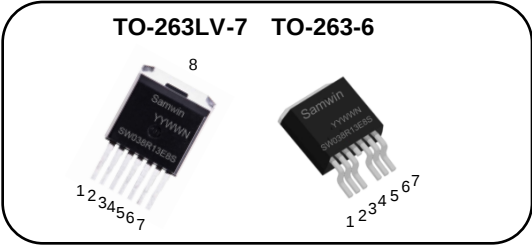
TO-263-7: 1. Gate 8.Drain 2-7.Source TO-263-6: 1. Gate 4.Drain 2,3,5-7.Source
