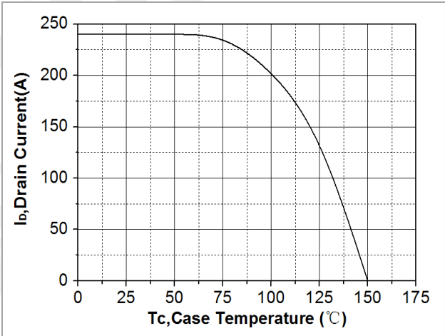
Fig. 10. Maximum drain current vs. case temperature (TO-263/TO-220)
