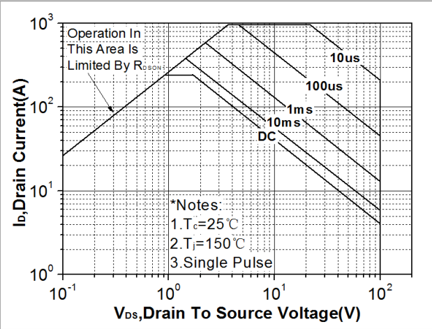
Fig. 9. Maximum safe operating area (TO-263/TO-220)
