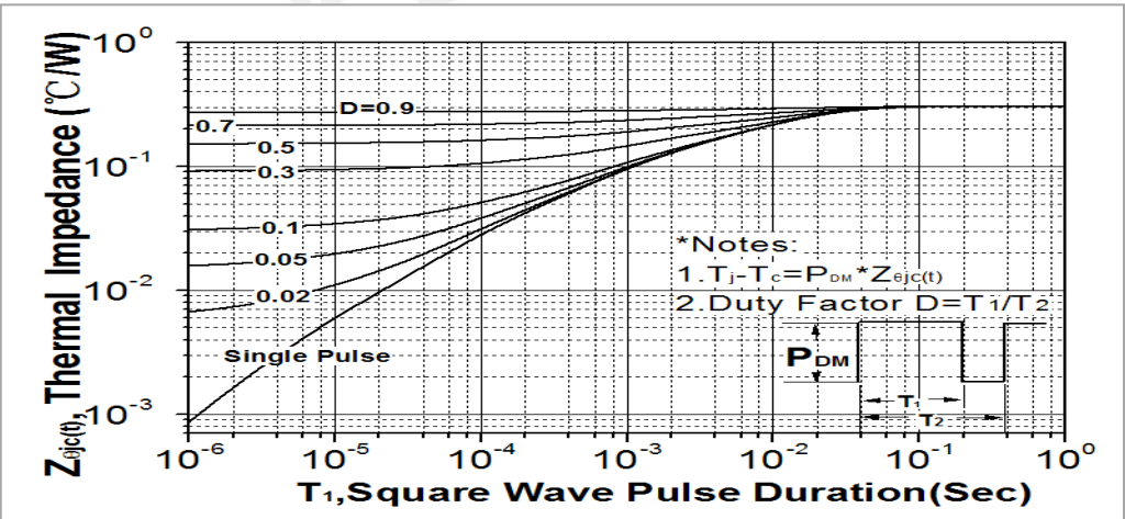
Fig. 11. Transient thermal response curve (TO-263/TO-220)
