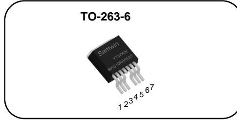
1. Gate 4.Drain 2,3,5~7.Source
