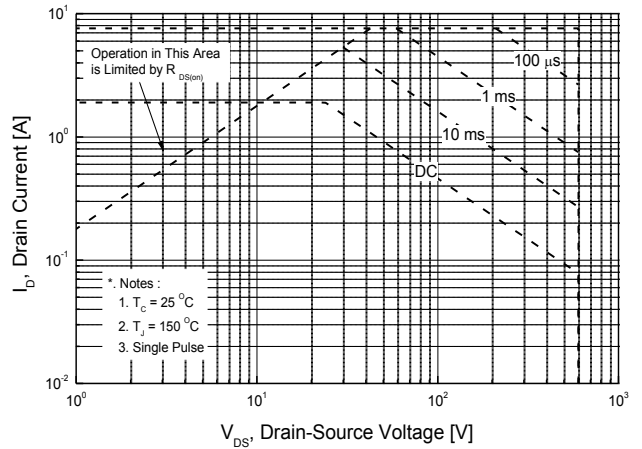
Fig. 10. Maximum safe operating area (TO-220)
