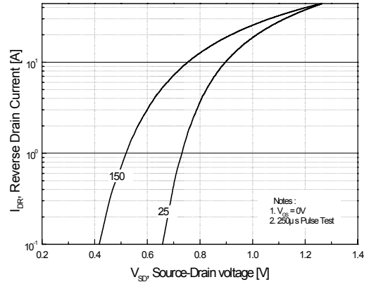
Fig. 4. On state current vs. diode forward voltage
