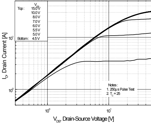
Fig. 1. On-state characteristics
